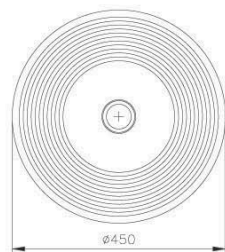
6510-05-8000 Glass Basin 450*140mm
